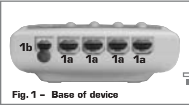
Fig. 1 – Base of device 1a Sockets for the four electrode cables 1b Socket for the battery charger
